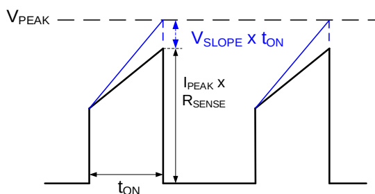
Figure 14: Typical Peak-Current Comparator
