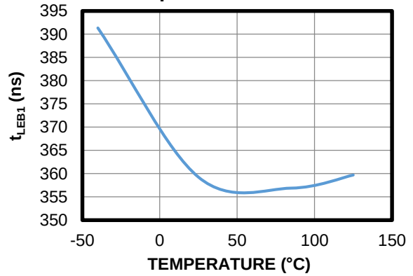
Leading Edge Blanking for V_{ILIMIT} vs. Temperature
