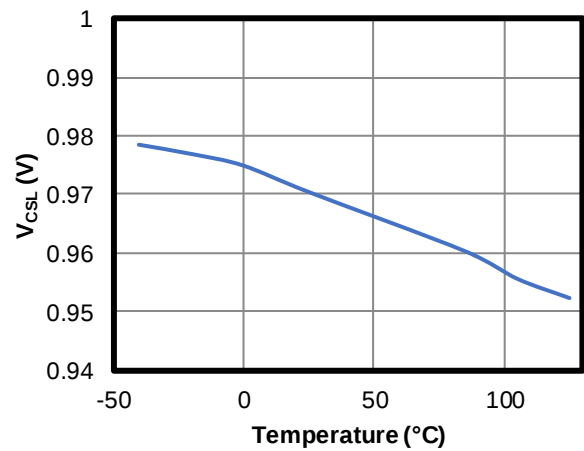
V_{CSL} vs. Temperature
