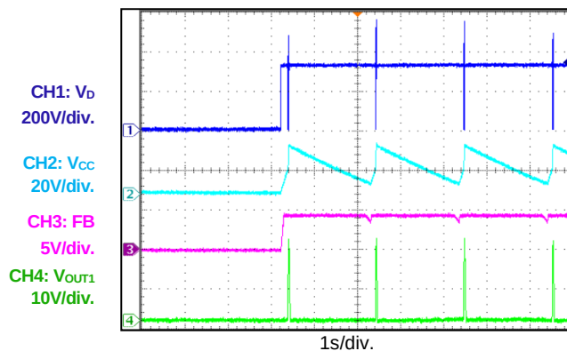
OVP Start-Up
