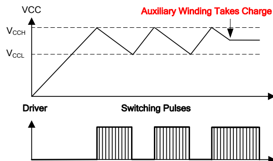
Figure 2: VCC Start-Up
