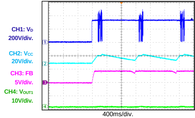
Short-Circuit Start-Up
