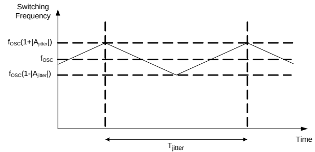
Figure 3: Frequency Jittering
