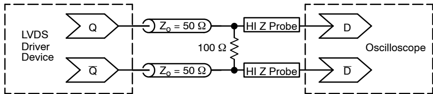
Figure 3. Typical Termination for Output Driver and Device Evaluation
