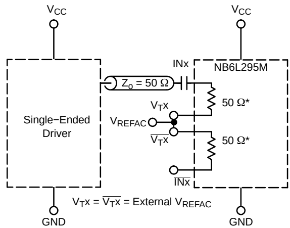
Figure 21. Capacitor-Coupled Single-Ended Interface ( V_{TX}/\sqrt{I_{TX}} Connected to External V_{REFAC} ; V_{REFAC} Bypassed to Ground with 0.1 \mu\text{F} Capacitor)
