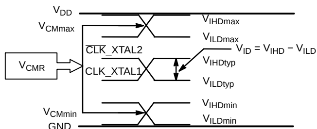
Figure 7. V_{CMR} Diagram
