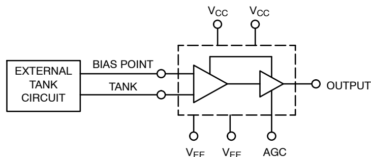
Figure 1. Logic Diagram
