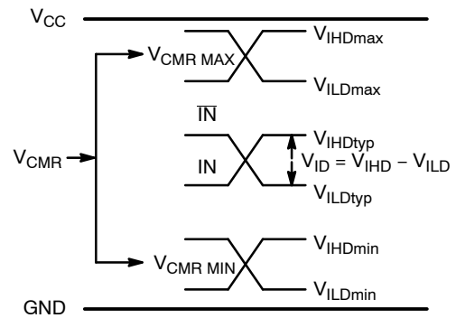
Figure 7. V CM Diagram
