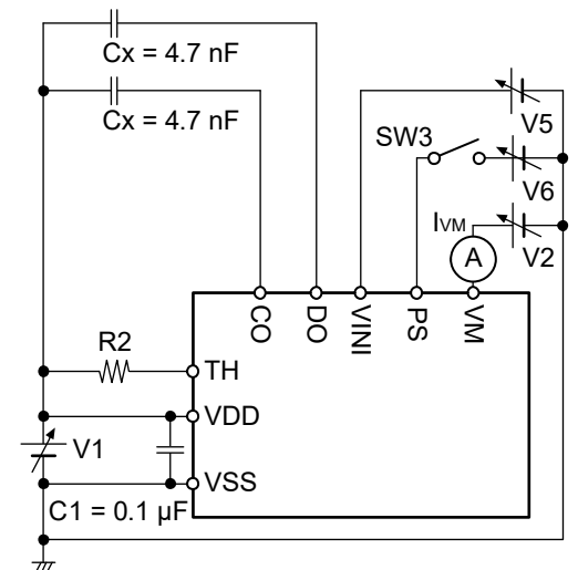
Figure 8 Test Circuit 4
