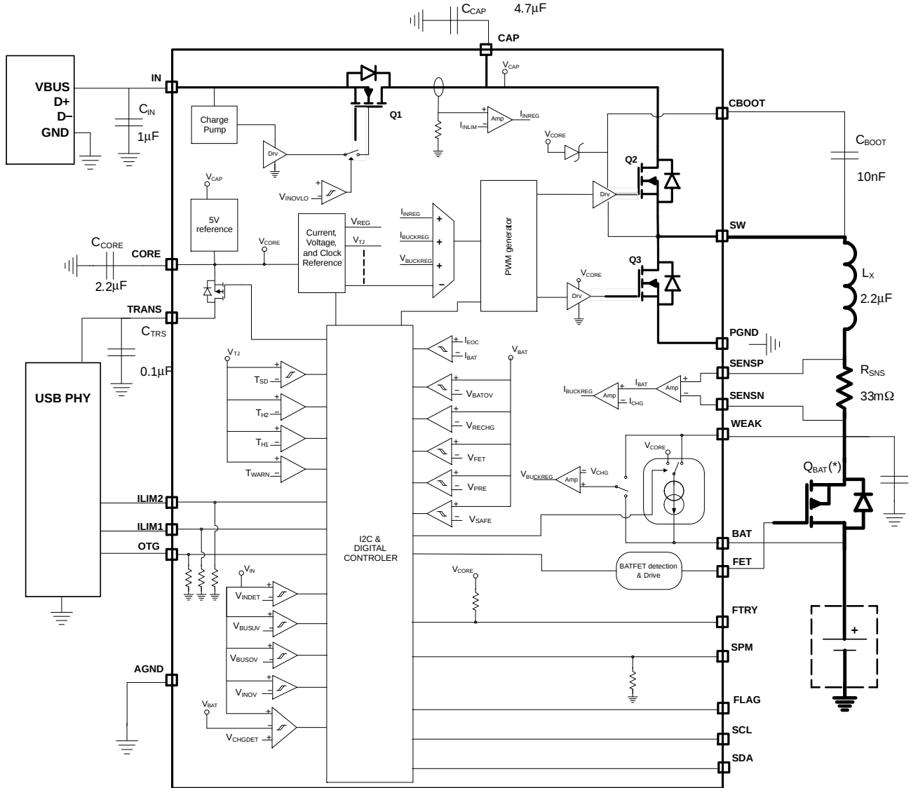
Figure 4. Block Diagram
