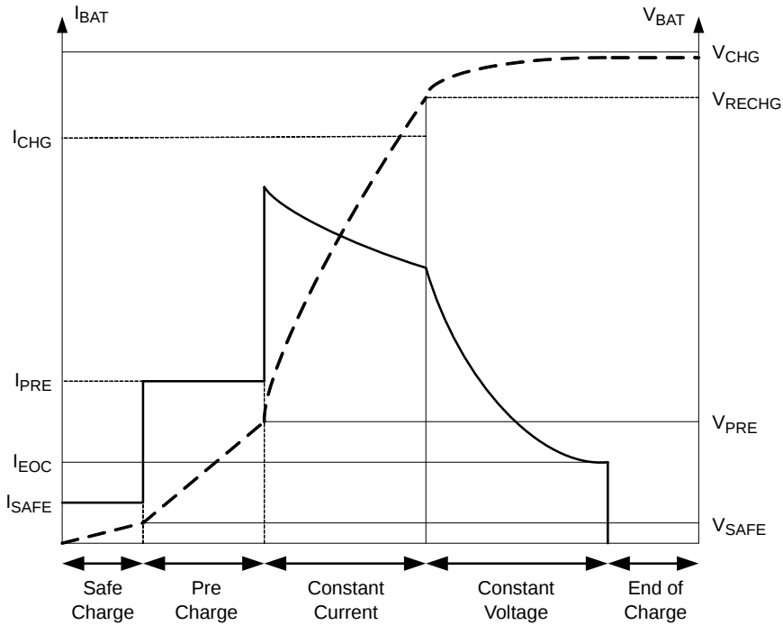
Figure 15. Typical Charging Profile of NCP1854 with Input Current Limit
