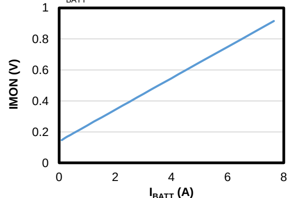
IMON Indicating I BATT in Discharge Mode
