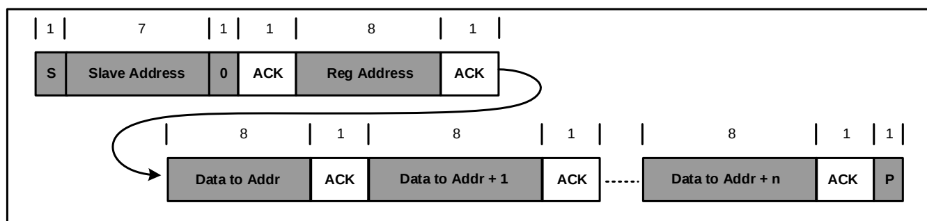
Figure 17: I²C Multi-Write
