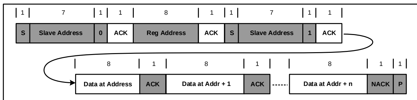
Figure 18: I²C Multi-Read
