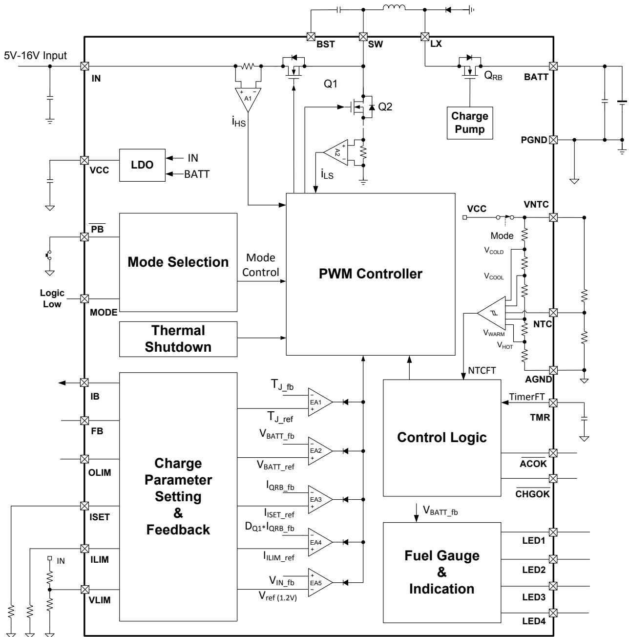
Figure 1: Block Diagram for Charge Mode
