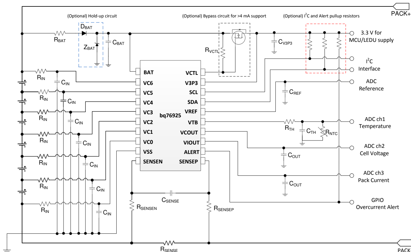
Figure 16. Typical Schematic
