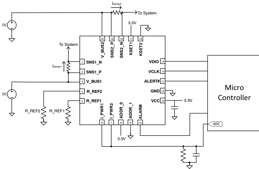
Figure 2. Application Schematic
