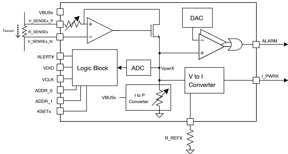
Figure 1. Block Diagram
