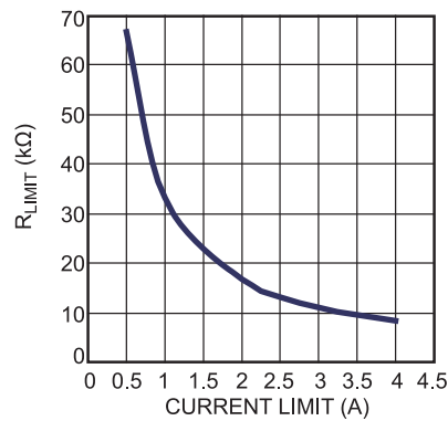
Current Limit vs. R_{LIMIT}
