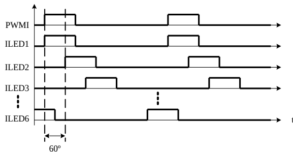
Figure 4: Phase Shift with 6 Channels
