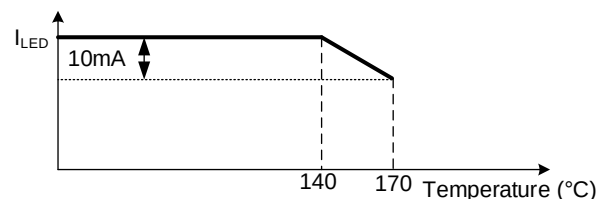
Figure 6: ILED Decrease with Temperature
