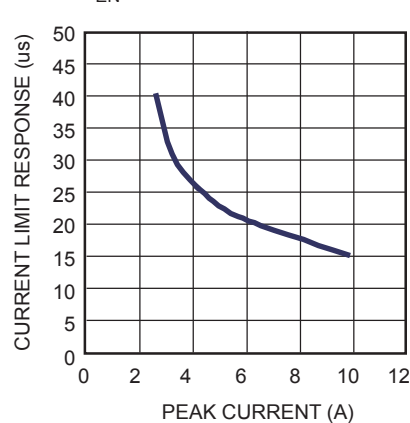
Current Limit Response Time vs. Peak Current
