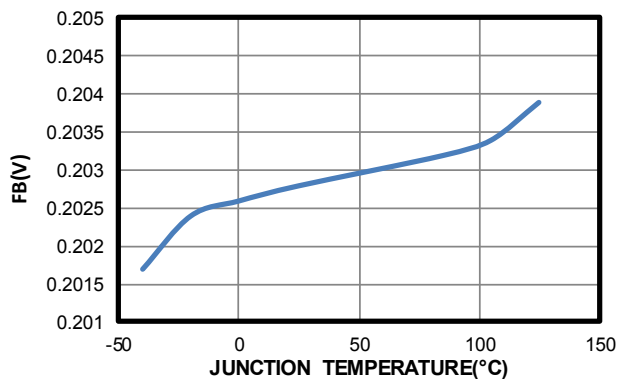
FB Reference Voltage vs. Junction Temperature
