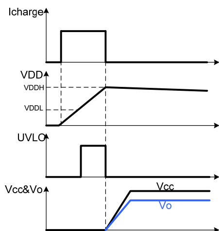
Figure 2: Start-Up Sequence
