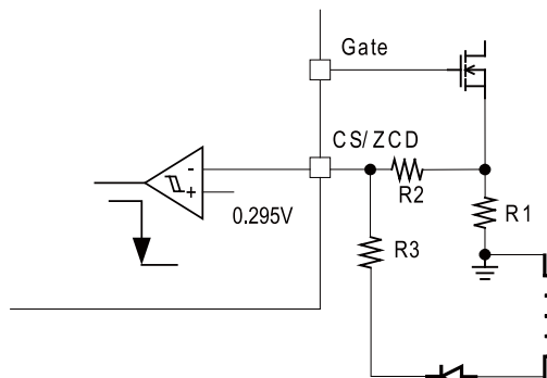
Figure 3: Zero-Current Detector
