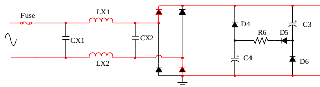
Figure 7: Stage A of Valley Fill Circuit
