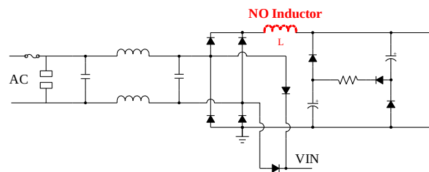
Figure 13: EMI Structure
