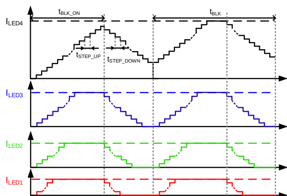
Figure 10: I_{LEDx} under Breathing Light
