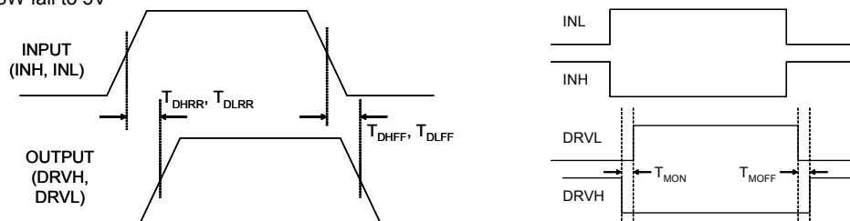
Figure 1—Timing Diagram
