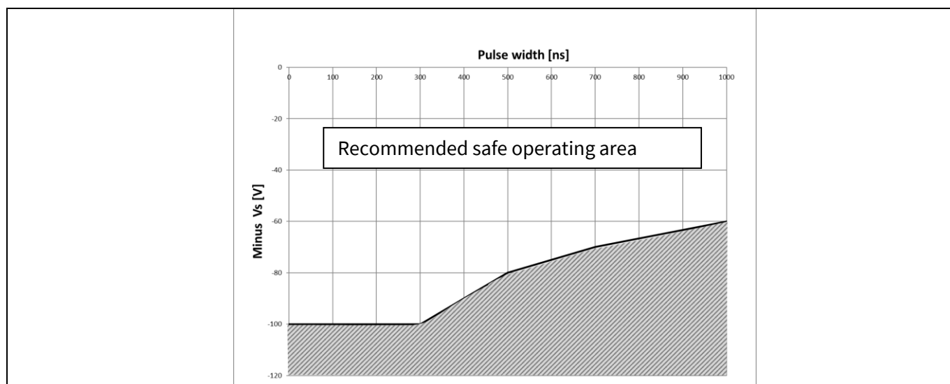
Figure 20 Negative VS transient SOA for 2ED2104S06F @ V_{BS}=15\text{ V}
