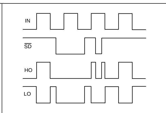
Figure 7 Input/output logic diagram
