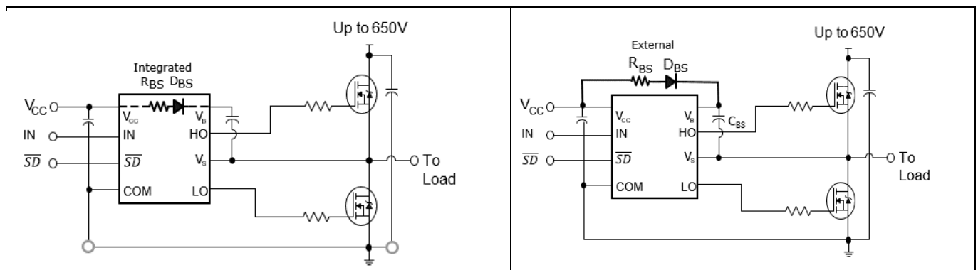
Figure 13 2ED210x with integrated components
