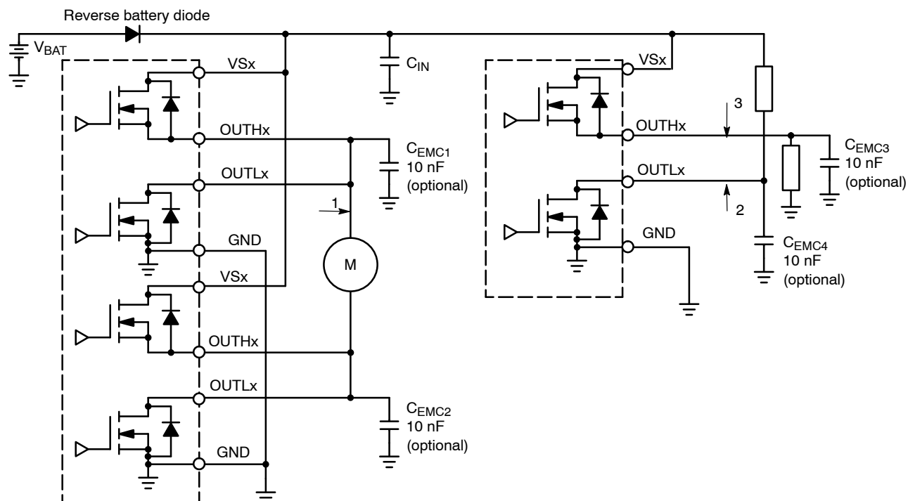
Figure 8. Application Drawing
