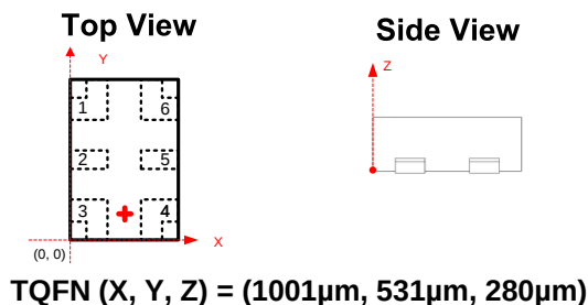
Figure 9: Hall Sensor Position
