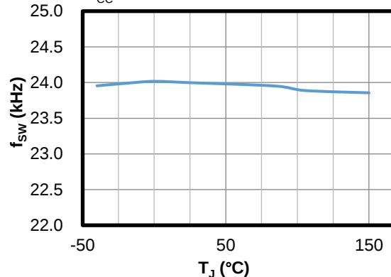
Switching Frequency vs. T_J
