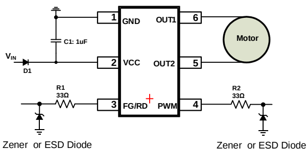
Figure 12: Enhanced ESD Using a Zener Diode or ESD Diode
