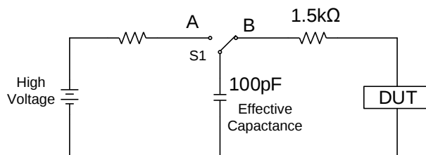
Figure 10: Equivalent Circuit of an HBM ESD Circuit
