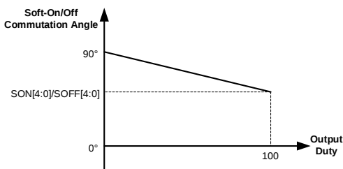
Figure 5 Soft-On/Off Commutation Angle Linear Interpolation
