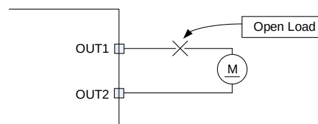
Figure 3: Half-Bridge Open Load Example
