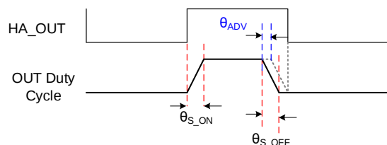
Figure 5: Advanced Soft-Off Angle
