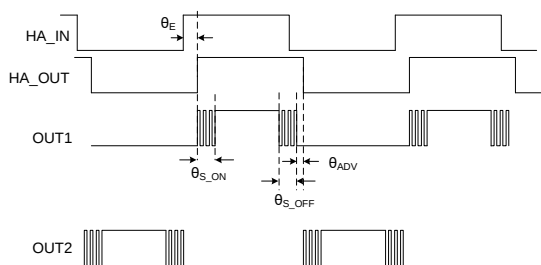
Figure 3: Operation Sequence
