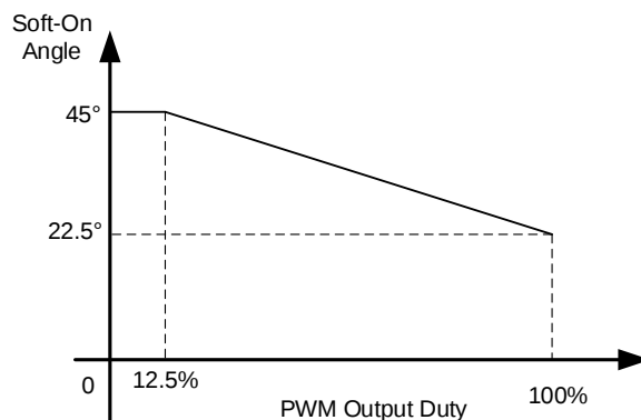
Figure 3: Soft-On Angle vs. Output Duty
