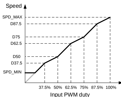
Figure 5: Curve Configuration when SPD_ZERO = 0
