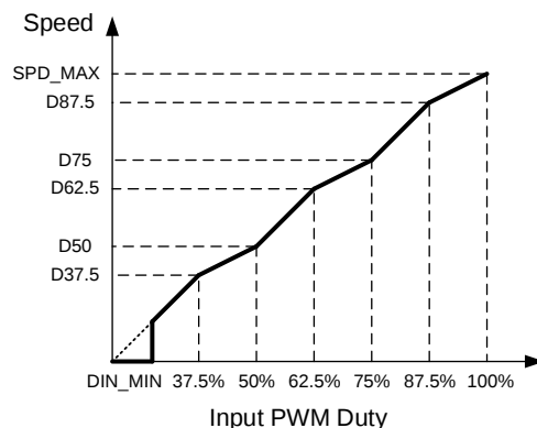
Figure 4: Curve Configuration when SPD_ZERO = 1
