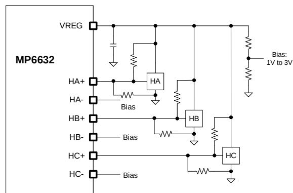
Figure 9: Hall-Sensor IC Connection with Differential Input Mode
