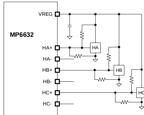
Figure 10: Hall-Sensor IC Connection with High/Low Logic Input Mode
