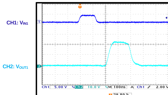
HS-FET Minimum On Time
