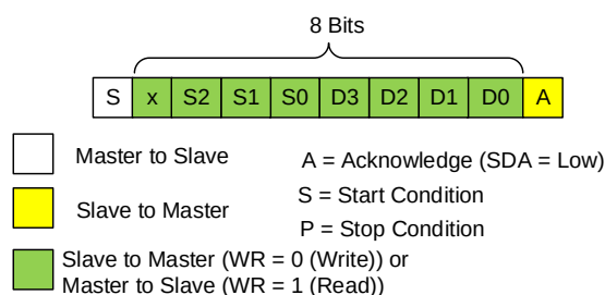
Figure 4: Data Byte
