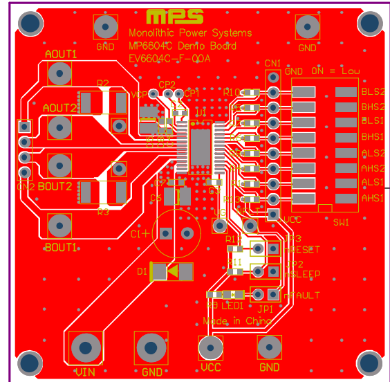
Figure 3: Recommended PCB Layout (MP6604CGF)
