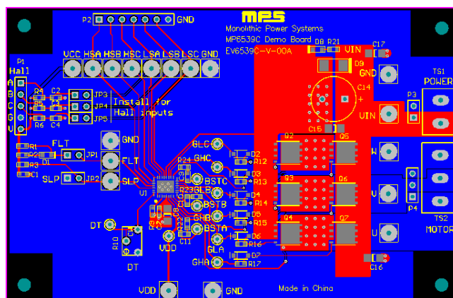
Figure 2: Recommended PCB Layout
