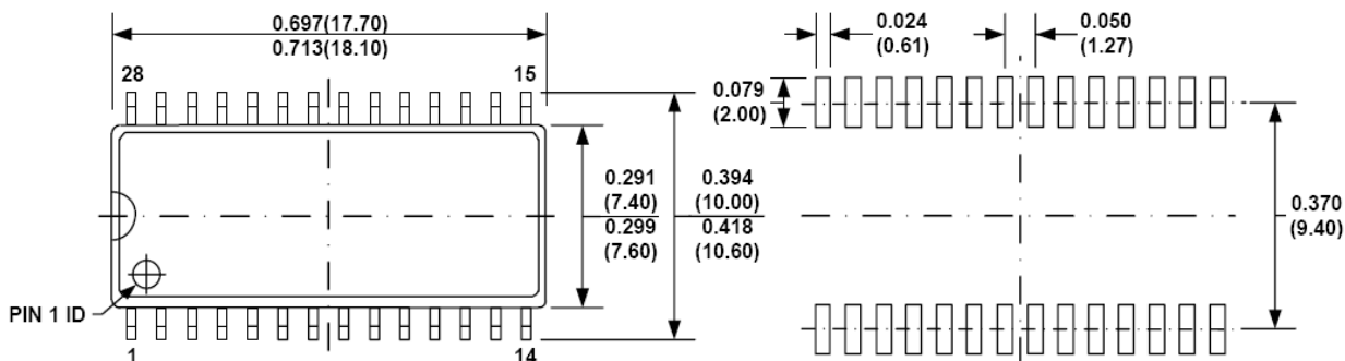
TOP VIEW
