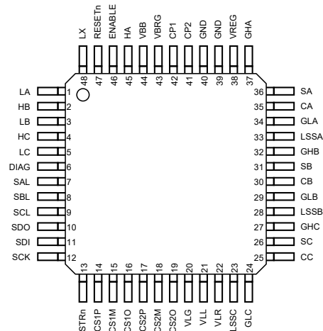
QFP-48 (JP) Package Pinout Diagram
