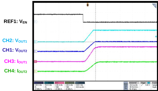
CH1/CH2 Start-Up through EN I_{OUT1} = 3A , I_{OUT2} = 2A
