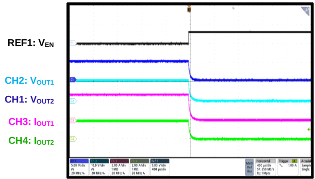
CH1/CH2 Shutdown through EN I_{OUT1} = 3A , I_{OUT2} = 2A
