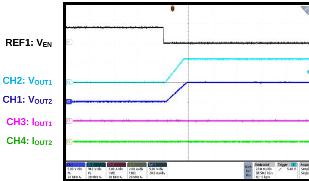
CH1/CH2 Start-Up through EN I_{OUT1} = I_{OUT2} = 0A
