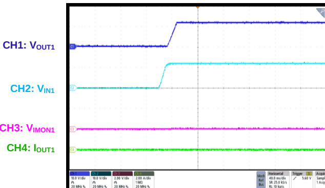
Start-Up through VIN1 12V e-fuse, no load
