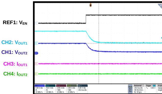
CH1/CH2 Shutdown through EN I_{OUT1} = I_{OUT2} = 0A
