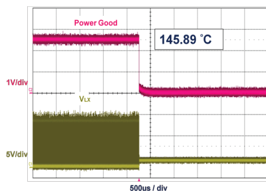
Fig. 22 - Thermal Shutdown - 146 °C ( V_{IN} = 12\text{ V} , V_{OUT} = 2.5\text{ A} to 10\text{ A} , di/dt = 1\text{ A}/\mu\text{s} )
