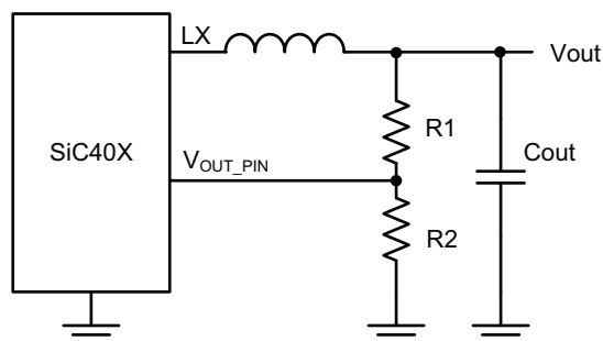
Fig. 40 - Resistor Divider Network allows 4.5 V at the V_{OUT} Pin
