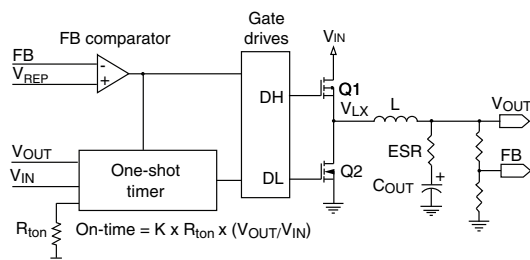
Fig. 24 - On-Time Generation
