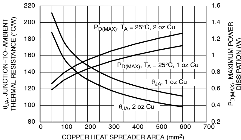
Figure 66. \theta_{JA} and P_{D(MAX)} vs. Copper Area (WDFN6)
