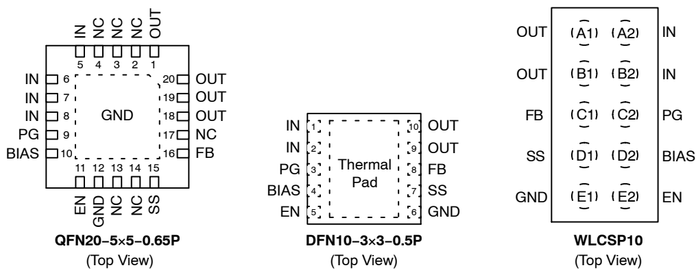
Figure 2. Pin Connections
