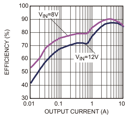
Figure 20 — Efficiency Curve
