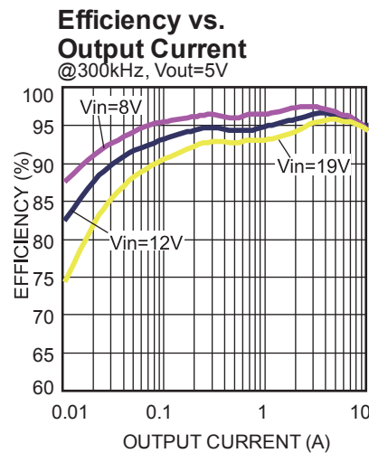
Figure 50 — Efficiency Curve
