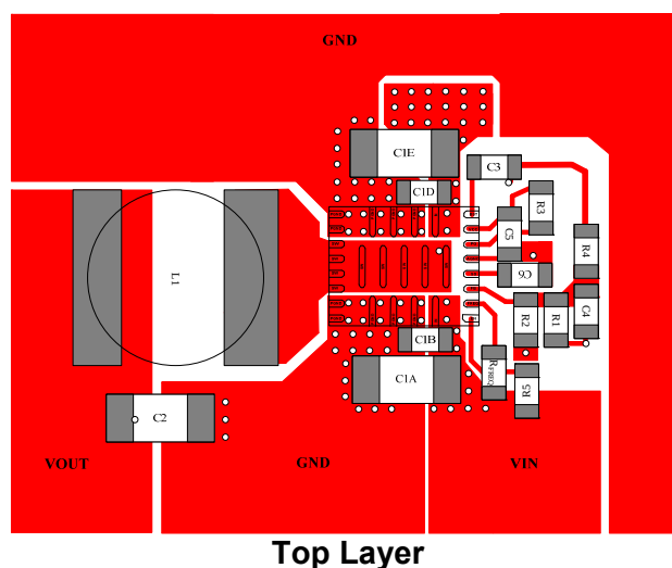
Figure 56—Recommend Input Capacitor Placement for 16-Pin QFN 3mmx4mm Package Part, including MPQ8632-4/6/8/10/12 and MPQ8632H-10.
