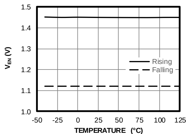
V_{EN} Threshold vs. Temperature
