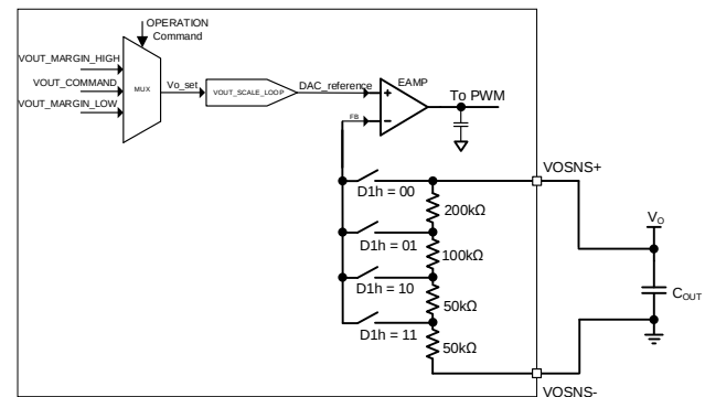
Figure 7: Output Voltage Set by Internal Resistor Divider
