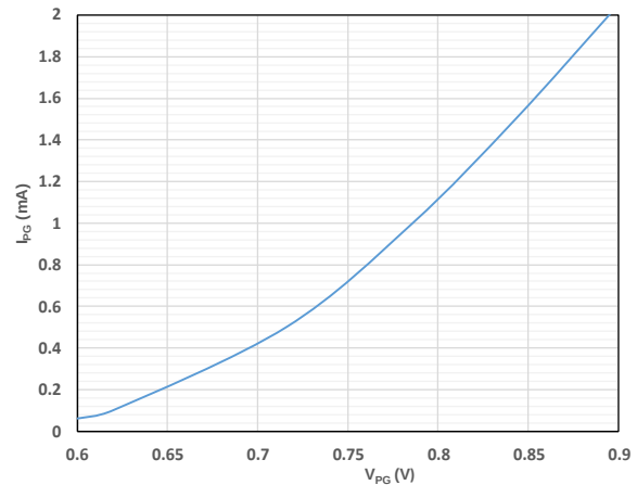
Figure 8: PGGOOD Clamped Voltage vs. Pull-Up Current
