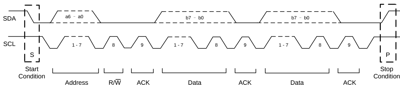
Figure 10: Data Transfer over PMBus
