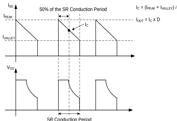
Figure 9: Synchronous Rectification Flyback Application
