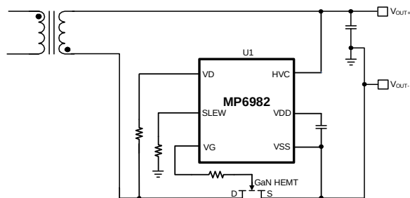
Figure 5: Low-Side Rectification
