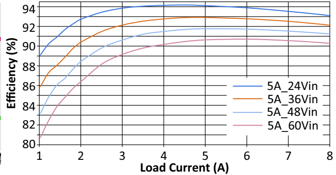
Figure 37. System Efficiency
