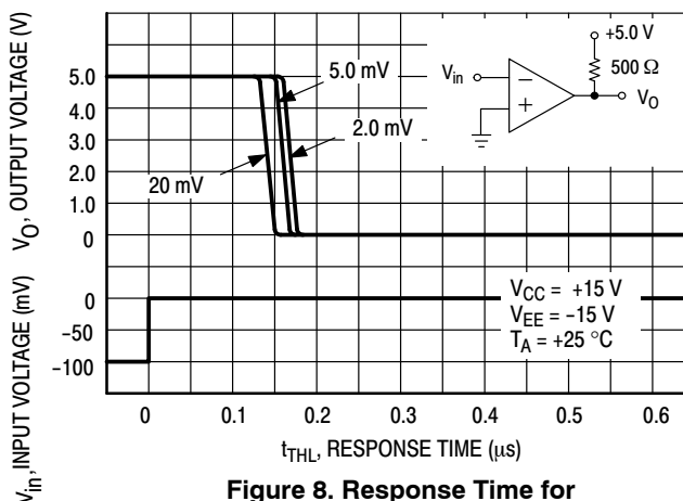
Figure 8. Response Time for Various Input Overdrives
