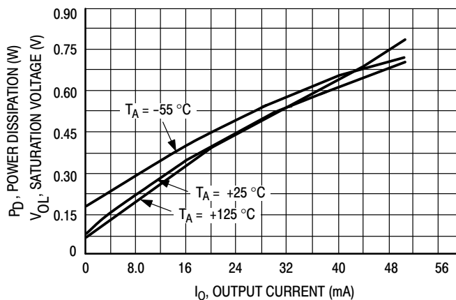
Figure 12. Output Saturation Voltage versus Output Current
