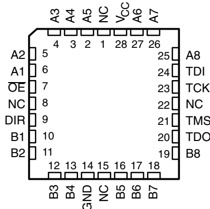
SN54BCT8245A . . . FK PACKAGE (TOP VIEW)
