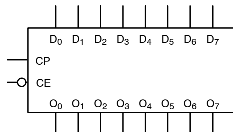
Figure 2. Logic Symbol
