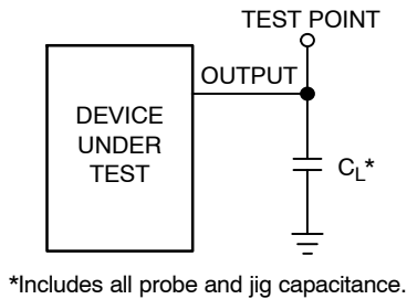
Figure 5. Test Circuit
